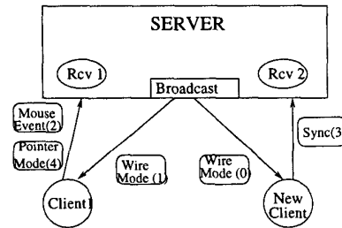
Figure 4: Synchronization of the System
