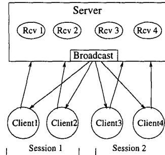
Figure 3: Client-Server Architecture
