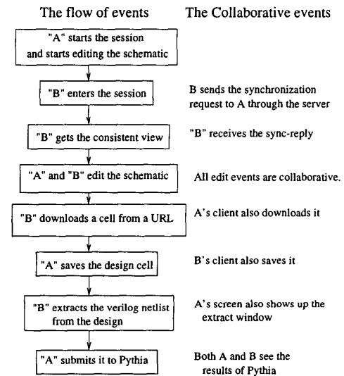
Figure 6: Example flow in CollabTop
