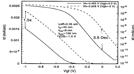
Figure 7: PMOS subthreshold characteristics.
