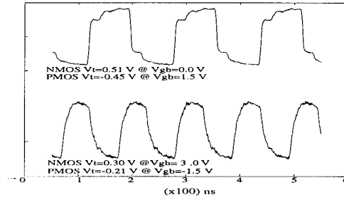
Figure 10: Ring oscillator output at different V_t 's tuned by back-gate bias.
