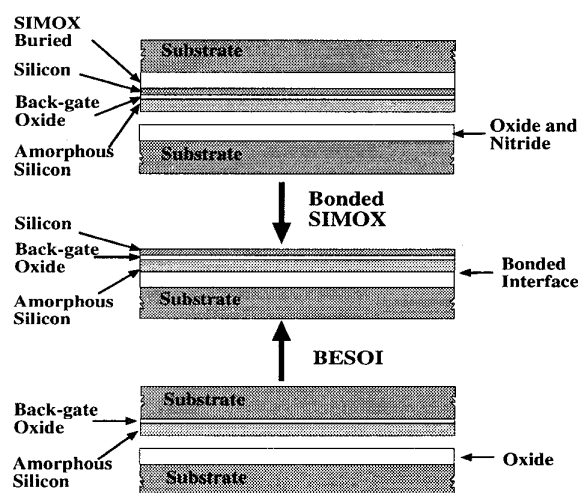
Figure 1: SOIAS preparation using bonded SIMOX and BESOI processes.
