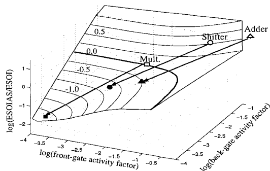
Figure 11: Energy ratio of SOI and SOIAS technologies for systems that are frequently in use (open symbols) and those that are mostly idle (2% usage for X server)(filled symbols).
