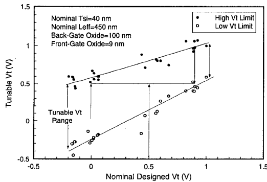
Figure 8: Tunable V_t ranges by back-gate biasing.
