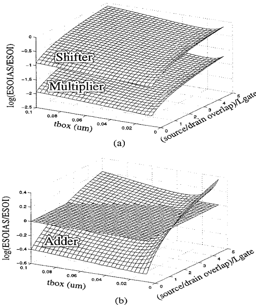
Figure 12: Energy ratio of SOI and SOIAS in the technology design space for functional modules with various activity factors.
