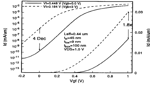
Figure 6: NMOS subthreshold characteristics.
