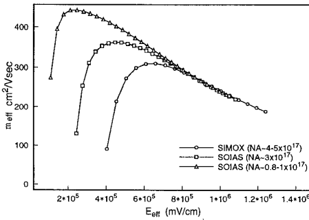
Figure 3: Effective electron mobility for SIMOX and SOIAS.
