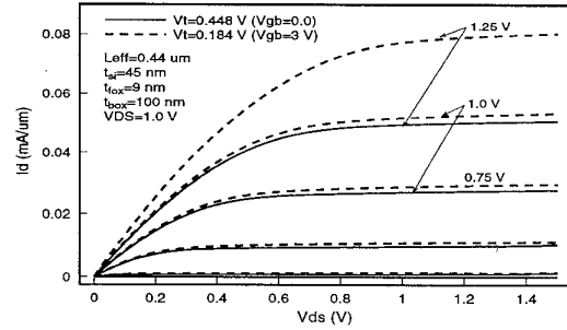
Figure 4: NMOS I-V tuned at different V_t 's.
