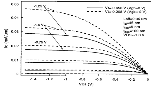
Figure 5: PMOS I-V tuned at different V_t 's.
