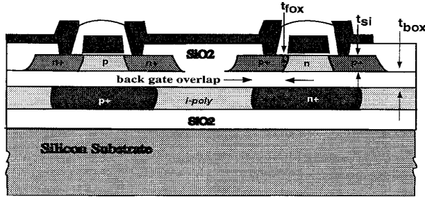
Figure 2: SOIAS back-gated CMOS device schematic.
