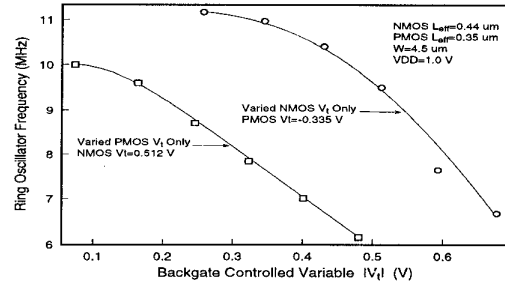
Figure 9: 101 stage ring oscillator output frequency as varied by changing V_t .
