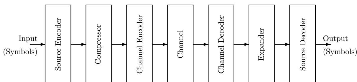
Figure 7.1: Communication system
