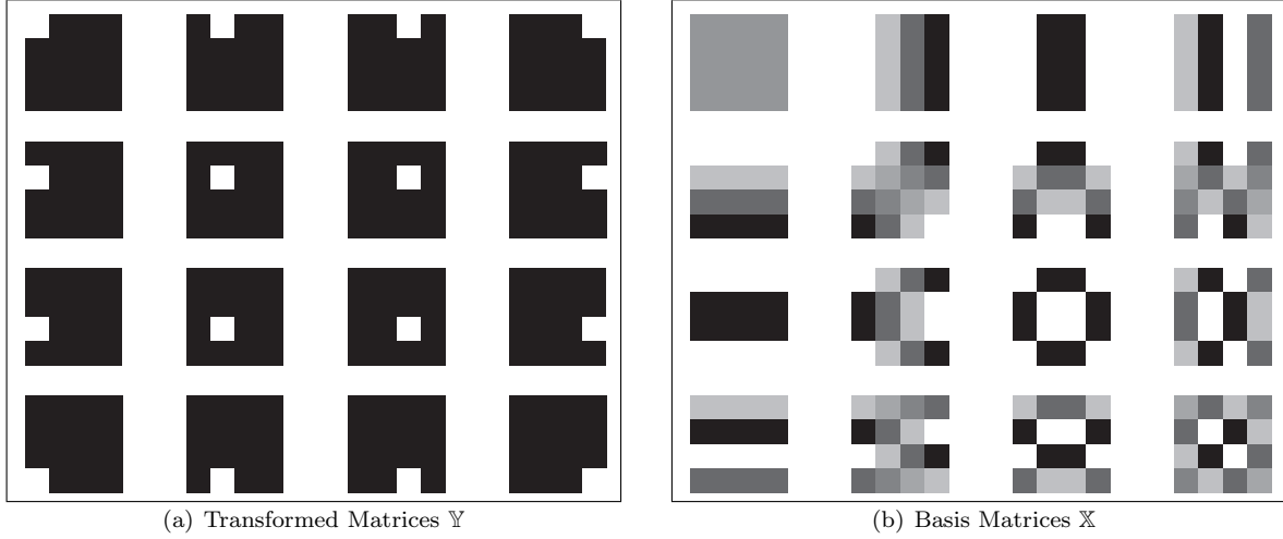
Figure 3.7: (a) 4 \times 4 pixel images representing the coefficients appearing in the matrix \mathbb{Y} from equation 3.15. And, (b) corresponding Inverse Discrete Cosine Transformations, these IDCTs can be interpreted as the base images that correspond to the coefficients of \mathbb{Y} .
