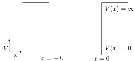
Figure 9-1: Infinite square well
