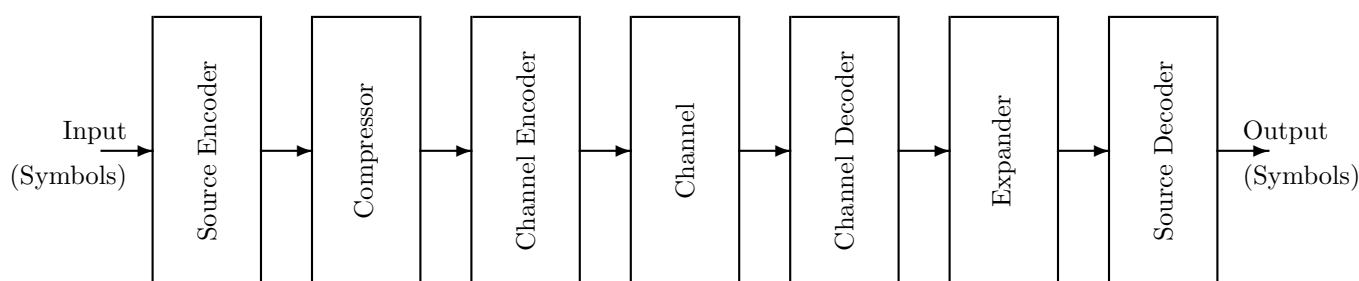
Figure 7.1: Elaborate communication system
